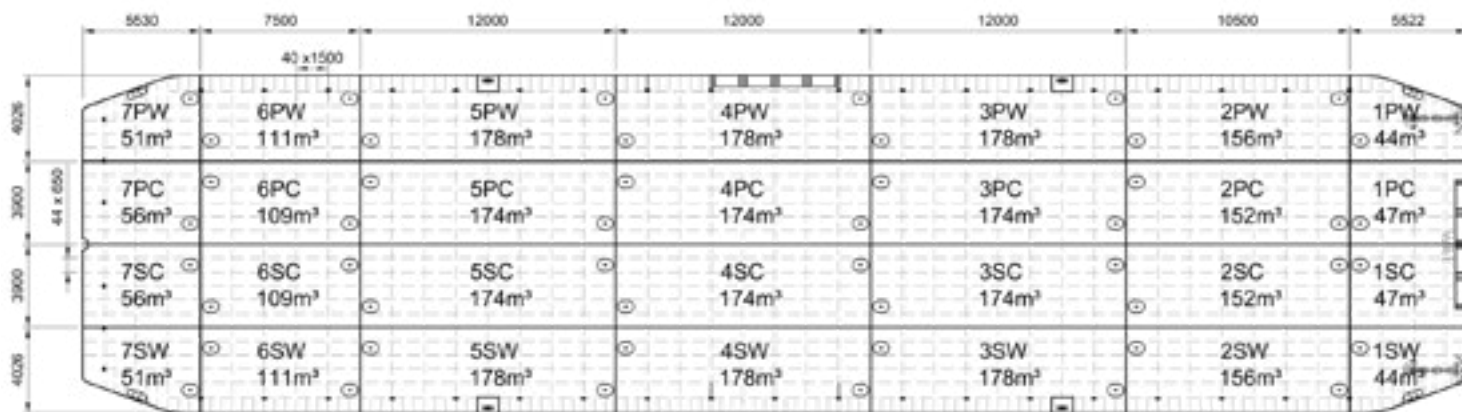
DECK AND STRUCTURAL LAYOUT
